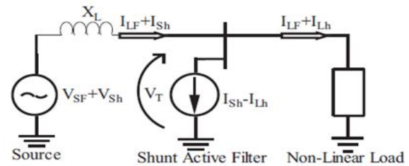
Fig.2 Principle of Shunt Current Compensation
