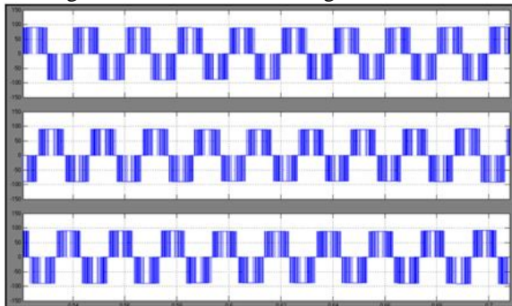
Fig.12 Three phase Voltage Generated by APF
