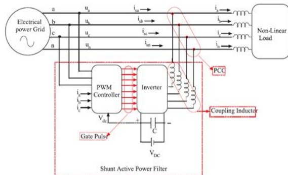
Fig.1 Shunt active power filters topology.
