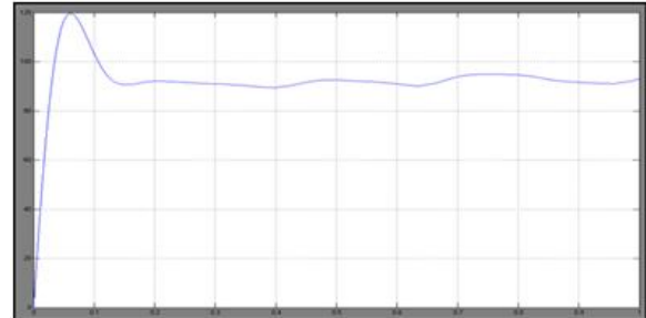
Fig.7 DC Capacitor Voltage During Switch-on Response with PI Controller
